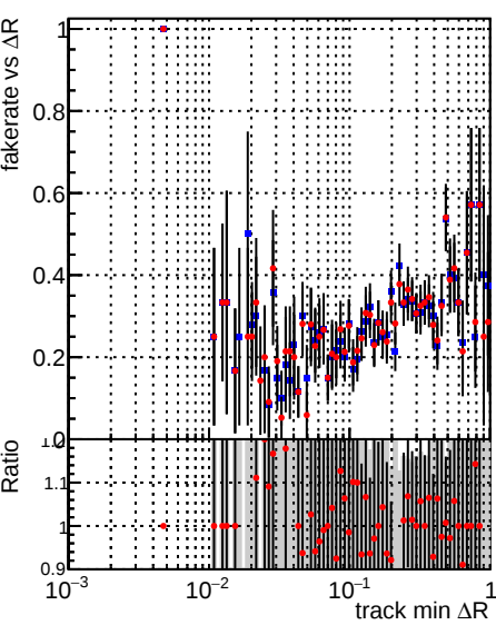
Fake rate vs ΔR(track, jet) DQM_TT_PR43146 DQM_TT_PR43146_swap
