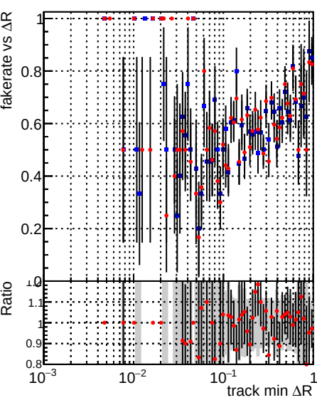
Fake rate vs \Delta R(\text{track, jet}) Legend: DQM_TT_PR43146 (blue dots), DQM_TT_PR43146_swap (red dots)
