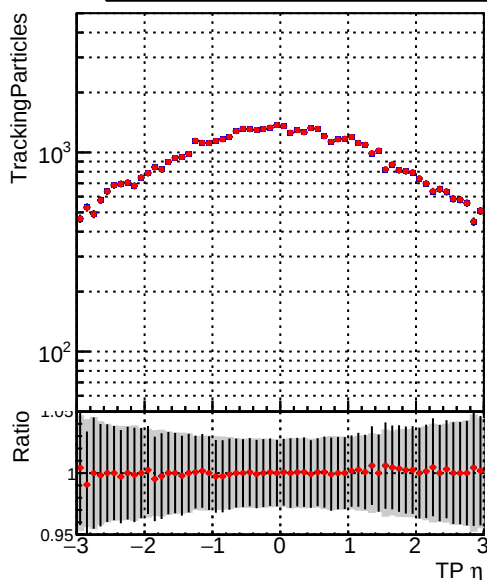
Legend: DQM_TT_PR43146 (blue squares), DQM_TT_PR43146_swap (red circles)
