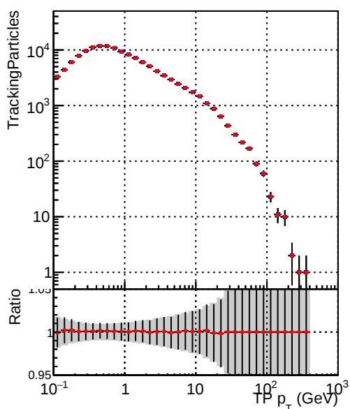
Legend: DQM_TT_PR43146 (blue squares), DQM_TT_PR43146_swap (red circles)
