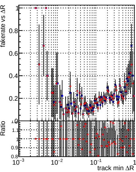
Fake rate vs \Delta R(\text{track, jet}) Legend: DQM_TT_PR43146 (blue), DQM_TT_PR43146_swap (red)
