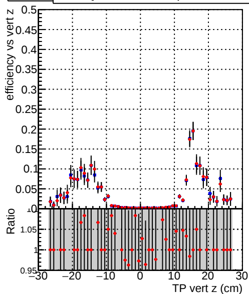
Efficiency vs vert z — DQM_TT_PR43146 — DQM_TT_PR43146_swap
