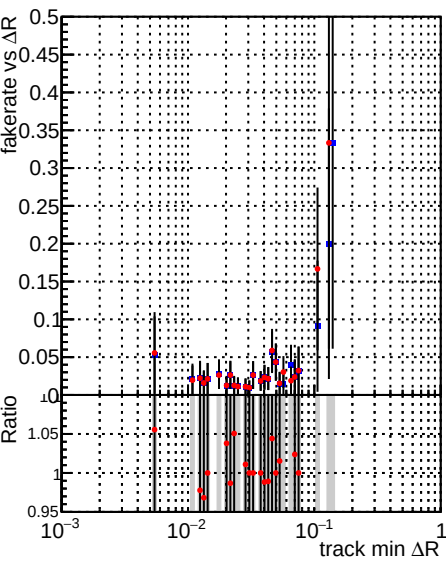
Fake rate vs ΔR(track, jet) DQM_TT_PR43146 DQM_TT_PR43146_material
