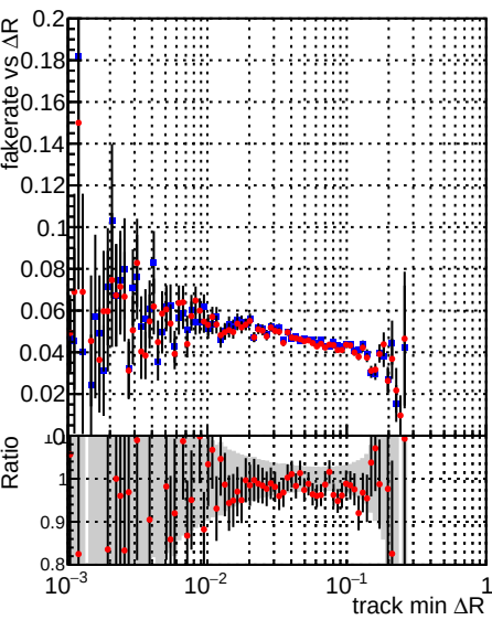
Fake rate vs \Delta R(\text{track}, \text{jet}) Legend: DQM_TT_PR43146 (blue), DQM_TT_PR43146_material (red)
