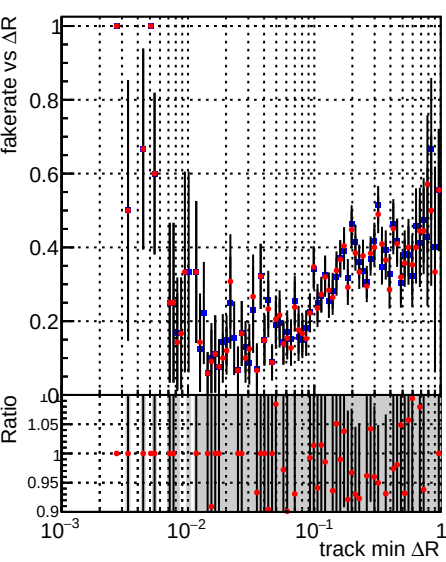
Fake rate vs \Delta R(\text{track, jet}) Legend: DQM_TT_PR43146 (blue stars), DQM_TT_PR43146_material (red stars)
