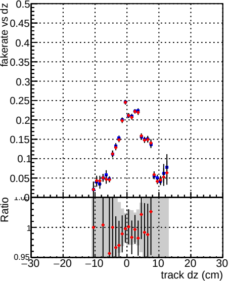
Fake rate vs dz Legend: DQM TT PR43146 (blue dots), DQM TT PR43146 material (red dots)
