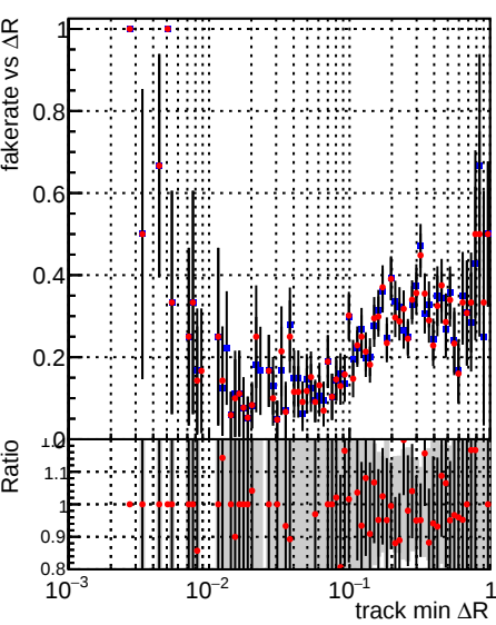
Fake rate vs \Delta R(\text{track, jet}) Legend: DQM_TT_PR43146 (blue squares), DQM_TT_PR43146_material (red circles)
