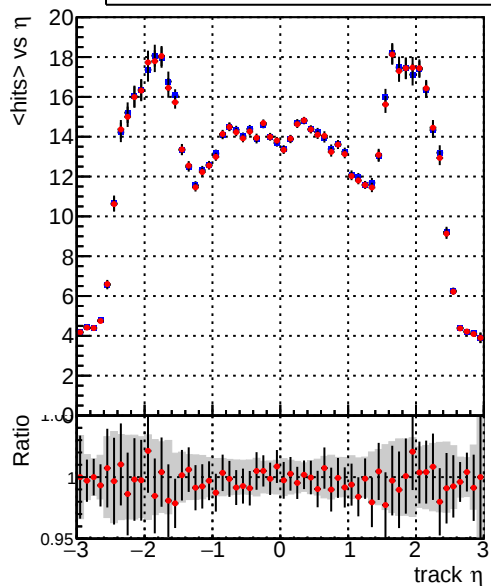
mean hits vs \eta — DQM_TT_PR43146 — DQM_TT_PR43146_material
