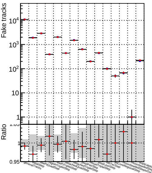
Number —●— DQM_TT_PR43146_material
