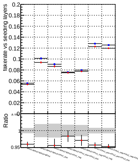
Fake rate vs. —●— DQM TT PR43146 —●— DQM TT PR43146 material
