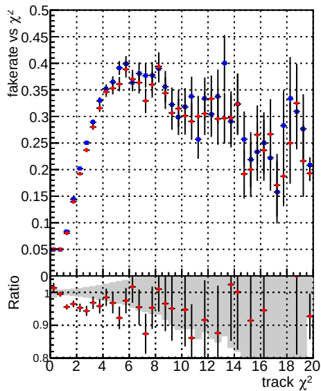
Fake rate vs. —●— DQM TT PR43146 —●— DQM TT PR43146 material
