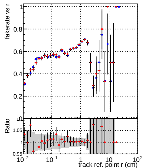
Fake rate vs verpos
