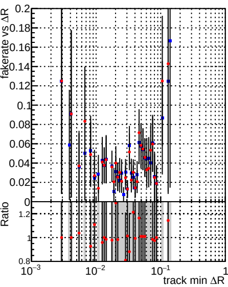
Fake rate vs \Delta R(\text{track, jet}) Legend: DQM_TT_PR43146 (blue), DQM_TT_PR43146_material (red)
