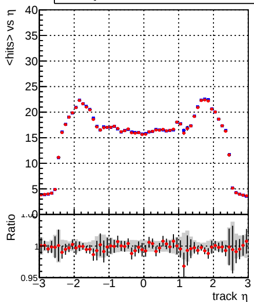
mean hits vs \eta Legend: DQM_TT_PR43146 (blue line), DQM_TT_PR43146_material (red line)
