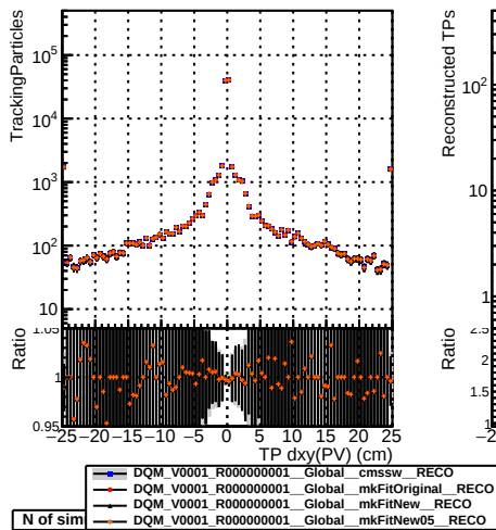
N of simulated tracks vs dxy(PV)
