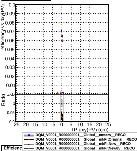
Efficiency vs Dxy(PV)
