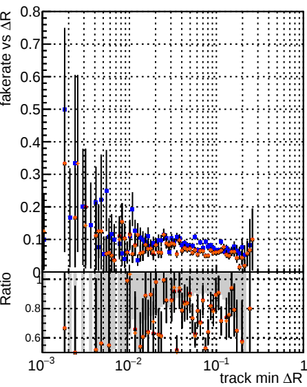
Fake rate vs \Delta R(\text{track, jet}) Legend: Global crossw RECO (blue stars) Global mkt0 Original RECO (orange stars) Global mkt1 New05 RECO (red stars)
