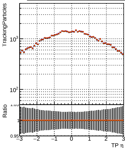
—●— DQM_V0001_R0000000001_Global_cmssw_RECO —●— DQM_V0001_R0000000001_Global_mkFitOriginal_RECO —●— DQM_V0001_R0000000001_Global_mkFitNew_RECO —●— DQM_V0001_R0000000001_Global_mkFitNew05_RECO
