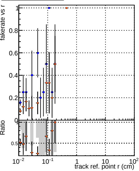
Fake rate vs v Legend: Global crossw RECO Global mkt0 Original RECO Global mkt0 New05 RECO
