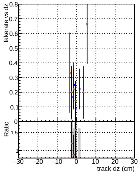
Fake rate vs d DGM V0001 B00000000001 Global cmsaw RECO DGM V0001 B00000000001 Global Original RECO DGM V0001 B00000000001 Global InNew RECO DGM V0001 B00000000001 Global InNew05 RECO
