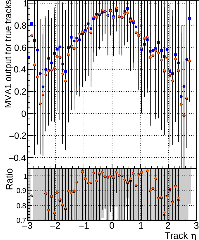
MVA1 of associated tracks (recoToSim) vs. track \eta ■ DQM_V0001_R0000000001 Global cmssw_RECO ● DQM_V0001_R0000000001 Global mkFitOriginal_RECO ▲ DQM_V0001_R0000000001 Global mkFitNew_RECO ★ DQM_V0001_R0000000001 Global mkFitNew05_RECO
