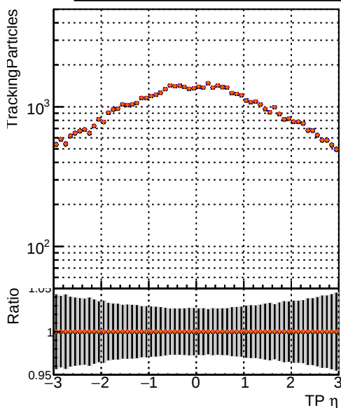
—●— DQM_V0001_R000000001_Global_cmssw_RECO —●— DQM_V0001_R000000001_Global_mkFitOriginal_RECO —●— DQM_V0001_R000000001_Global_mkFitNew_RECO —●— DQM_V0001_R000000001_Global_mkFitNew05_RECO
