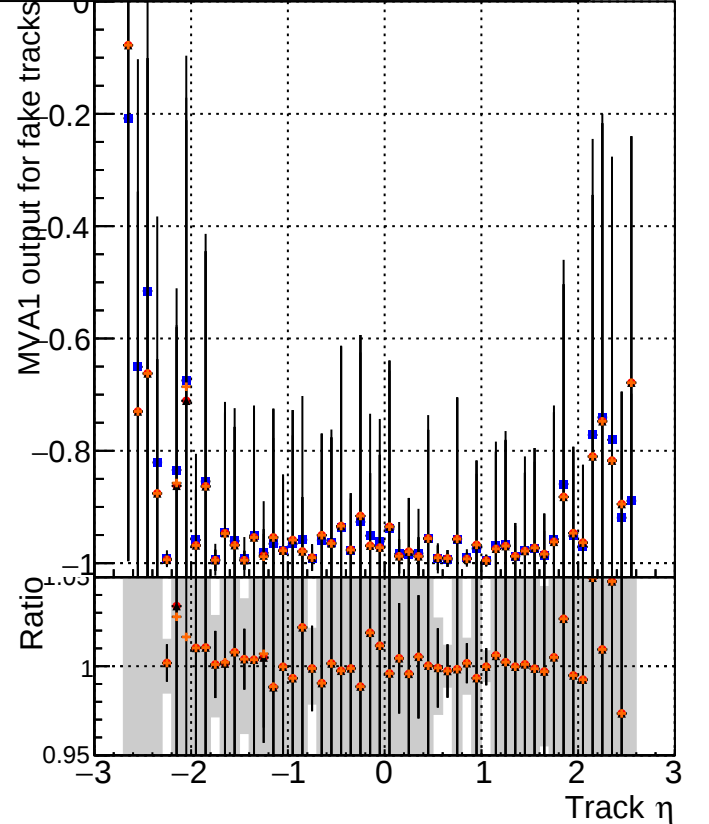
MVA1 of associated tracks (recoToSim) vs. track \eta Legend Series Global Model Blue square DQM_V0001_R0000000001 Global cmssw_RECO Red circle DQM_V0001_R0000000001 Global mkFitOriginal_RECO Black triangle DQM_V0001_R0000000001 Global mkFitNew_RECO Orange star DQM_V0001_R0000000001 Global mkFitNew05_RECO
