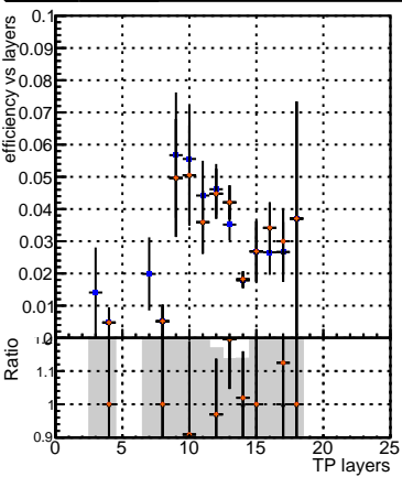
Efficiency vs hit —◆— DQM_V0001_R000000001_Global_cmssw_RECO —●— DQM_V0001_R000000001_Global_mkFitOriginal_RECO —▲— DQM_V0001_R000000001_Global_mkFitNew_RECO —■— DQM_V0001_R000000001_Global_mkFitNew05_RECO
