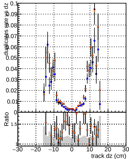
mkFitNew05 RECO
