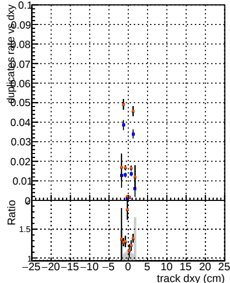
mkFitNew05 RECO
