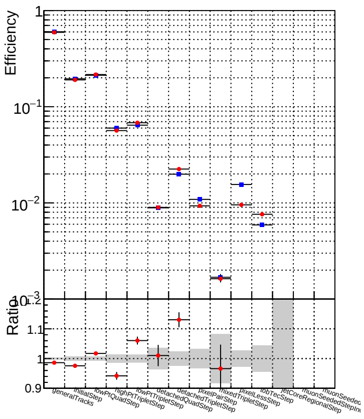
DQM_V0001_R000000001_Global_cmssw_RECO DQM_V0001_R000000001_Global_mkFitNew_RECO
