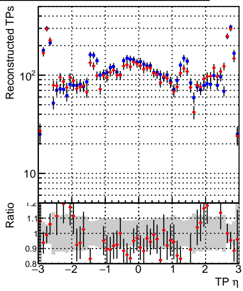
Legend: DQM_V0001_R000000001_Global_cmssw_RECO (blue squares), DQM_V0001_R000000001_Global_mkFitNew_RECO (red circles)
