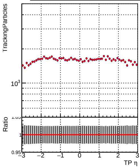
Legend: DQM_V0001_R0000000001_Global_cmssw_RECO (blue line), DQM_V0001_R0000000001_Global_mkFitNew_RECO (red line)
