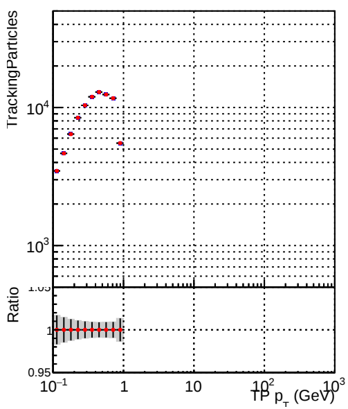
Legend: DQM_V0001_R0000000001_Global_cmssw_RECO (blue line), DQM_V0001_R0000000001_Global_mkFitNew_RECO (red line)
