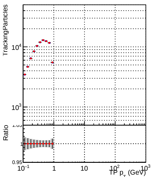
—•— DQM_V0001_R000000001_Global_cmssw_RECO —•— DQM_V0001_R000000001_Global_mkFitNew_RECO
