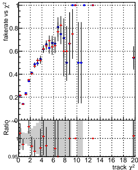
Fake rate vs. —●— DQM_V0001_R000000001_Global_cmssw_RECO —●— DQM_V0001_R000000001_Global_mkFitNew_RECO
