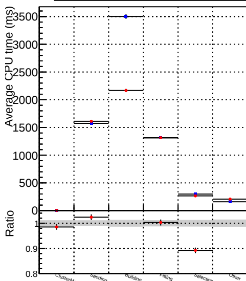
Average —●— DQM_V0001_R000000001_Global_mkFitNew_RECO
