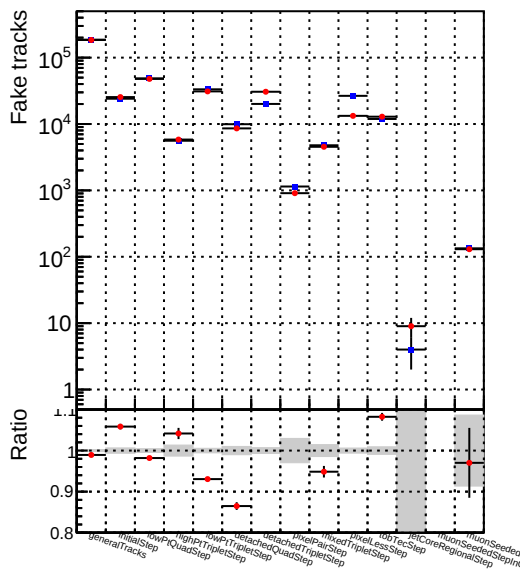
Number ● DQM_V0001_R000000001_Global_mkFitNew_RECO
