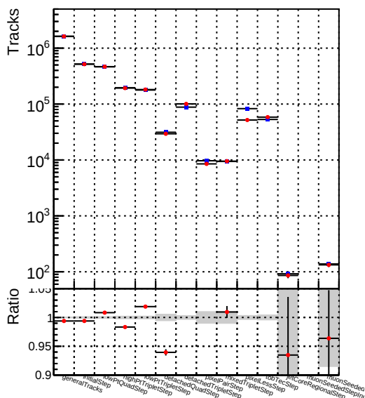
DQM_V0001_R000000001_Global_cmssw_RECO
