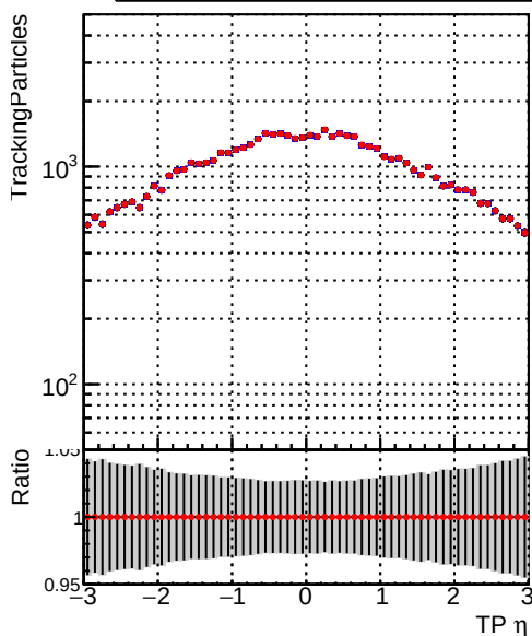
—•— DQM_V0001_R000000001_Global_cmssw_RECO —•— DQM_V0001_R000000001_Global_mkFitNew_RECO
