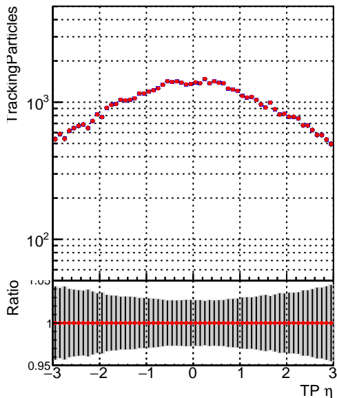
—●— DQM_V0001_R000000001_Global_cmssw_RECO —◆— DQM_V0001_R000000001_Global_mkFitNew_RECO
