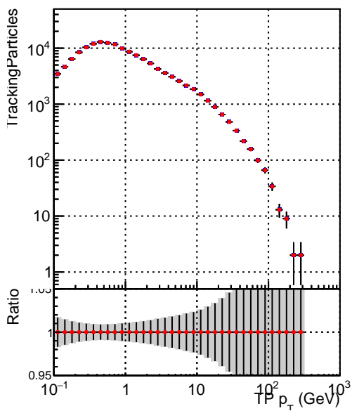
—●— DQM_V0001_R000000001_Global_cmssw_RECO —◆— DQM_V0001_R000000001_Global_mkFitNew_RECO
