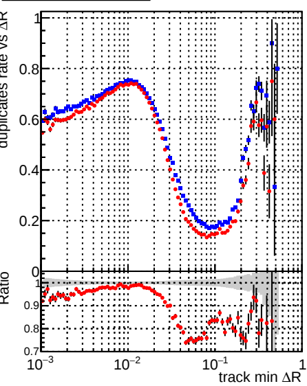
Legend: DQM_V0001_R000000001_Global_cmssw_RECO (blue line with dots), DQM_V0001_R000000001_Global_mkFitNew_RECO (red line with dots)
