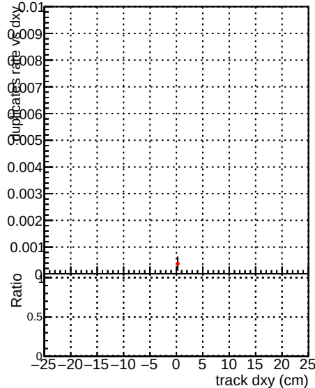
al_cmssw_RECO al_mkFitNew_RECO
