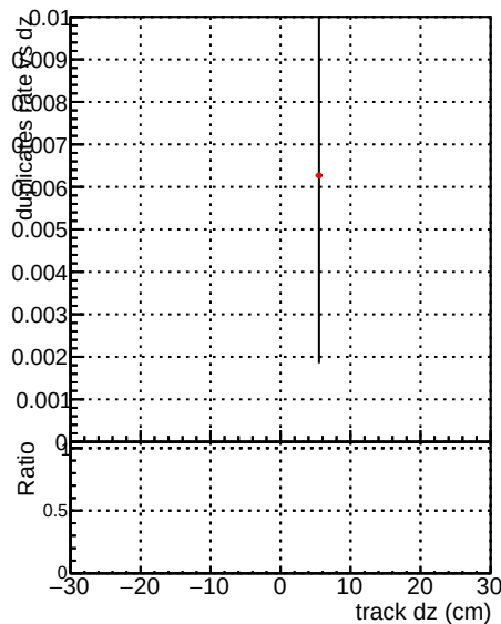
al_cmssw_RECO al_mkFitNew_RECO
