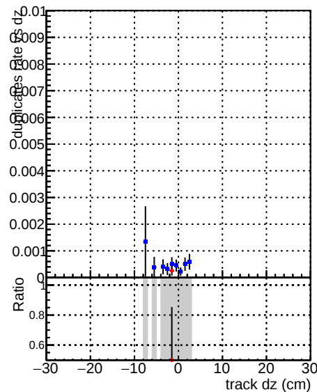
—●— DQM_V0001_R0000000001_Global_cmssw_RECO —●— DQM_V0001_R0000000001_Global_mkFitNew_RECO
