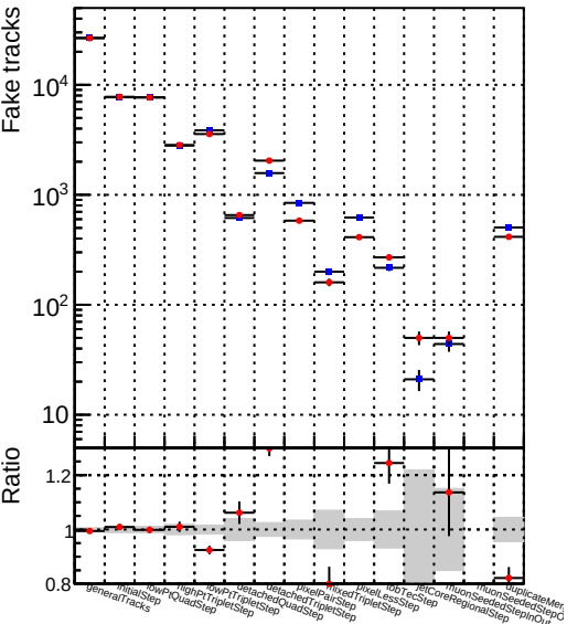
Numbe ● DQM_V0001 R000000001 Global mkFitNew RECO
