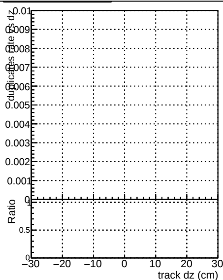
—•— DQM_V0001_R0000000001_Global_cmssw_RECO —•— DQM_V0001_R0000000001_Global_mkFitNew_RECO
