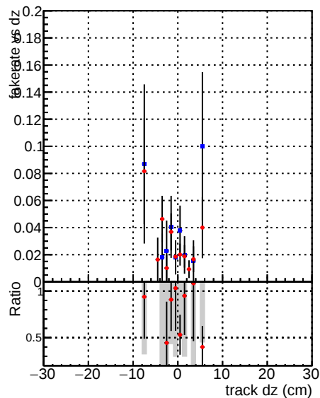
Fake rate vs dz Global cmssw_RECO Global mkFitNew_RECO
