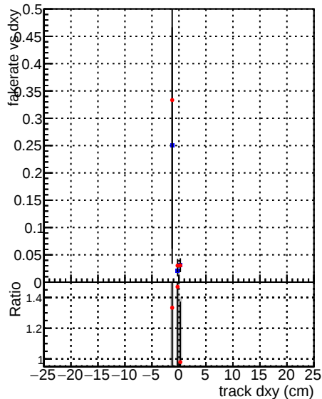
—●— DQM_V0001_R0000000001_Global_cmssw_RECO —●— DQM_V0001_R0000000001_Global_mkFitNew_RECO
