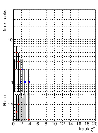
N of reco track vs. \chi^2 —●— DQM_V0001_R000000001_Global_cmssw_RECO —●— DQM_V0001_R000000001_Global_mkFitNew_RECO
