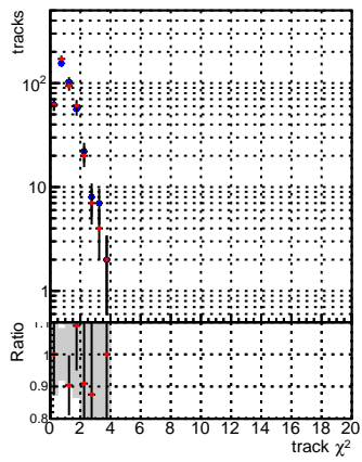
N of reco track vs. \chi^2 —●— DQM_V0001_R000000001_Global_cmssw_RECO —●— DQM_V0001_R000000001_Global_mkFitNew_RECO
