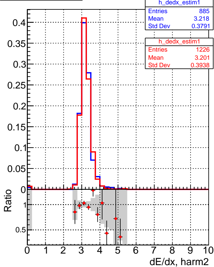
—■ DQM_V0001_R000000001_Global_cmssw_RECO —● DQM_V0001_R000000001_Global_mkFitNew_RECO
