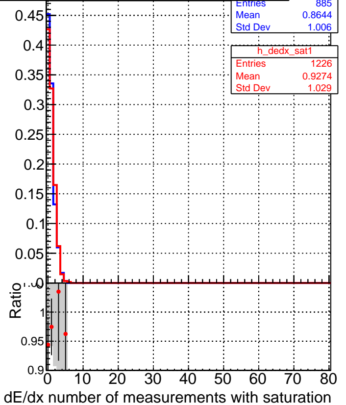
—■ DQM_V0001_R000000001_Global_cmssw_RECO —● DQM_V0001_R000000001_Global_mkFitNew_RECO
