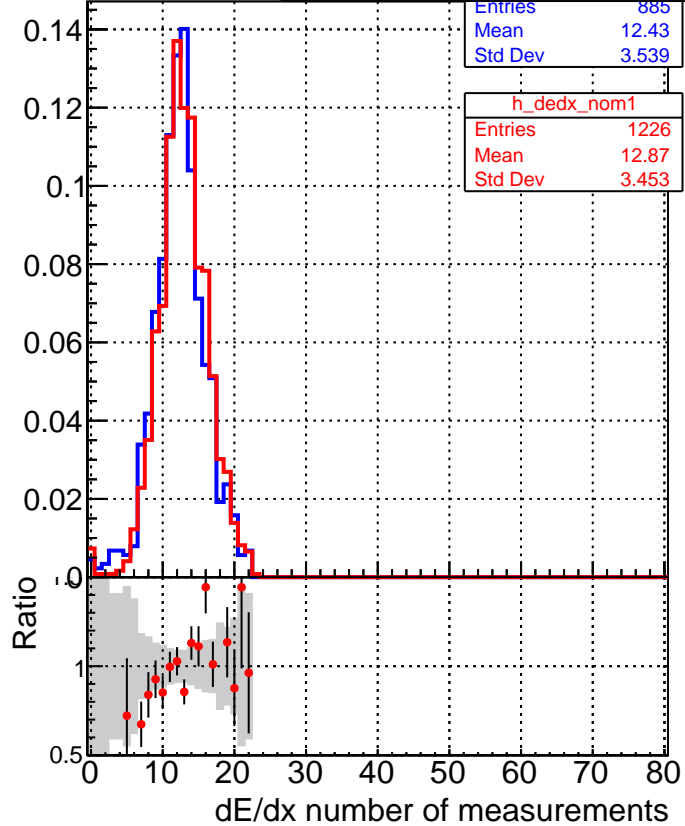
—■ DQM_V0001_R000000001_Global_cmssw_RECO —● DQM_V0001_R000000001_Global_mkFitNew_RECO
