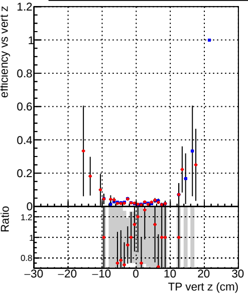
Efficiency vs TP vert z (cm) Legend: DQM_V0001_R000000001_Global_cmssw_RECO DQM_V0001_R000000001_Global_mkFitNew_RECO
