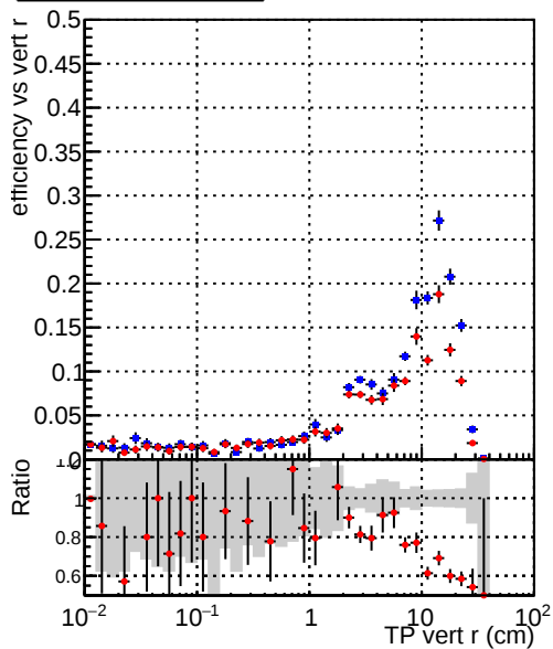
Efficiency vs verto r
