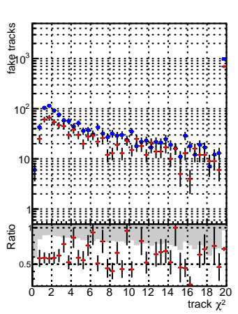
Legend: ● Global_cmssw_RECO ● Global_mkFitNew_RECO ● verBat
