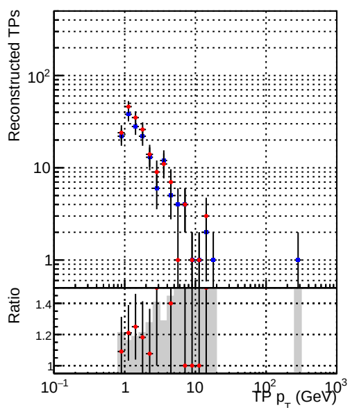
—•— DQM_V0001_R000000001_Global_cmssw_RECO —•— DQM_V0001_R000000001_Global_mkFitNew_RECO
