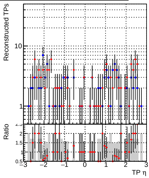
—•— DQM_V0001_R000000001_Global_cmssw_RECO —•— DQM_V0001_R000000001_Global_mkFitNew_RECO
