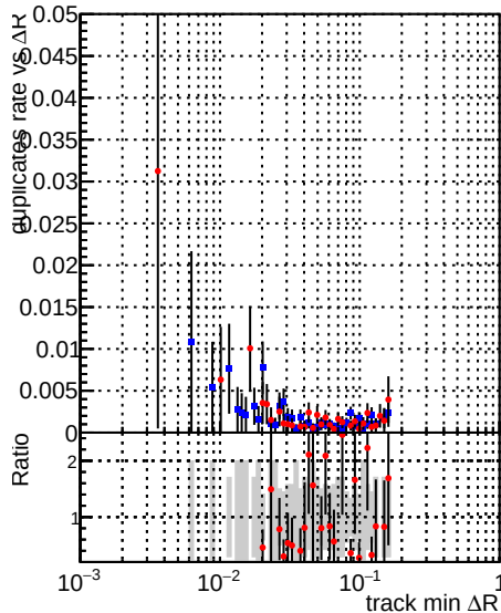
—●— DQM_V0001_R000000001_Global_cmssw_RECO —●— DQM_V0001_R000000001_Global_mkFitNew_RECO
