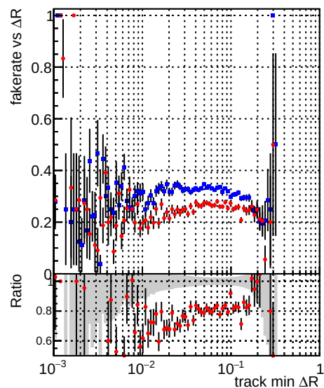
—●— DQM_V0001_R000000001_Global_cmssw_RECO —●— DQM_V0001_R000000001_Global_mkFitNew_RECO
